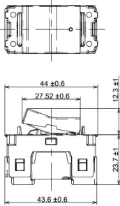
埋入式電鈴開關B
