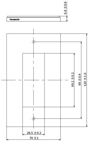
蓋板 (3個用)(附安裝框)
